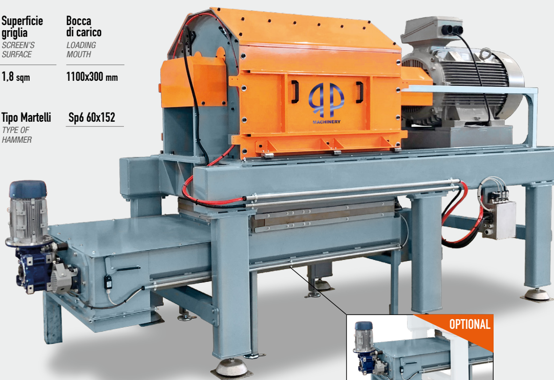
Scarico a coclee - Screws extractors unit
